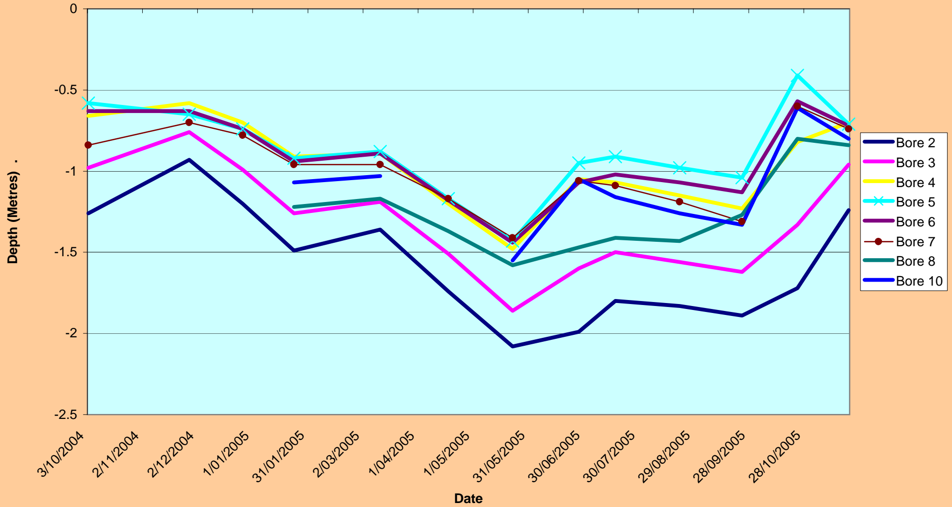
Kamarooka Watertable (Manual Measurements - Saline land bores only)
